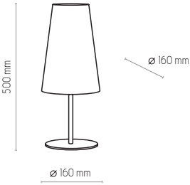
5171 | UMBRELLA | 1 x E27, 25W LED | AB 9090
