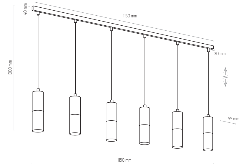
4358 | ELITE WHITE | 6 x GU10, 10W LED
