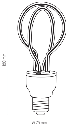
4370 | BULB LED | 230V 2200 K, E 27, 8W, 500lm, 50HZ
