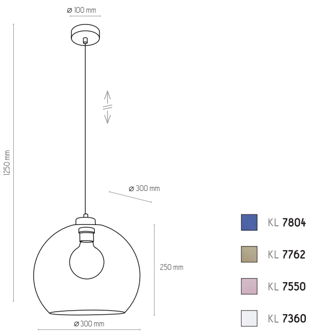
3174, 3161, 2764, 2742 | CUBUS | 1 x E27, max 60W
