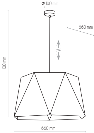
3129 | IVO | 1x E27, 25W LED | AB 9953
