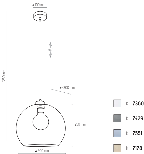
2076, 4292, 2765, 2064 | CUBUS | 1 x E27, max 60W
