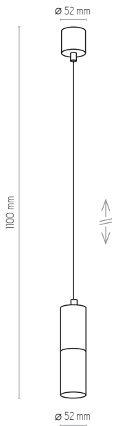
4356 | ELITE WHITE | 1 x GU10, 10W LED
