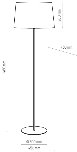
2919 | MAJA WHITE | 1x E27, 25W LED | AB 8407
