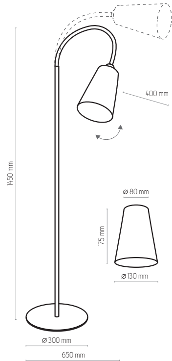
5166 | WIRE SILVER | 1 x E27, 15W LED | AB 9080
