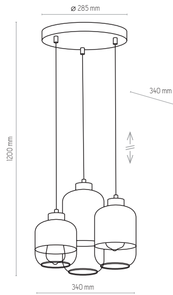
3357 | MARCO SILVER | 3 x E27, max 60W
