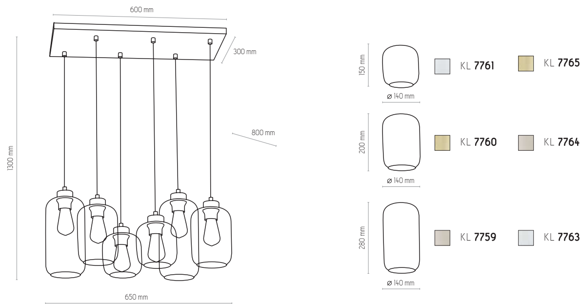
3176 | MARCO BROWN | 6 x E27, max 60W
