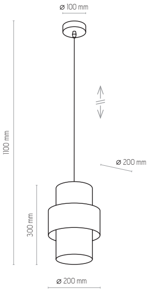
4377 | CALISTO | 1 x E27, 15W LED | AB 9083
