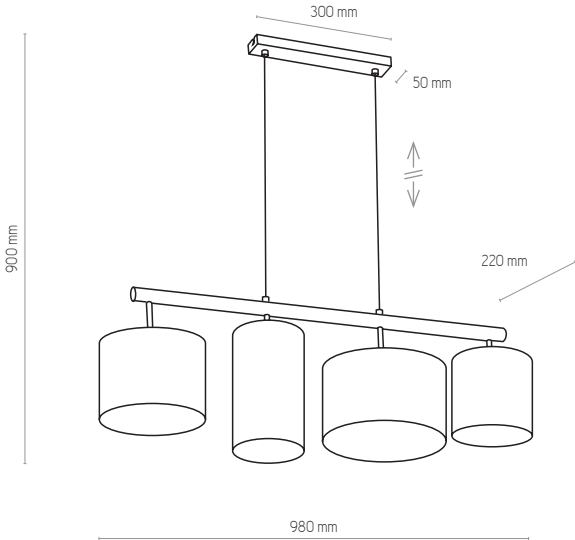
4458 | DEVA GRAPHITE | 4 x E27, 15W LED | AB 8940
