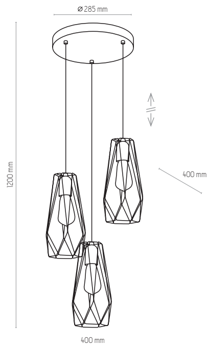
2697 | LUGO GOLD | 3 x E27, max 60W | DM 52
