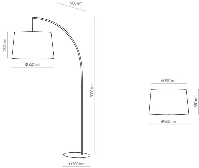
5076 | HANG | 1x E27, 25W LED | AB 8409
