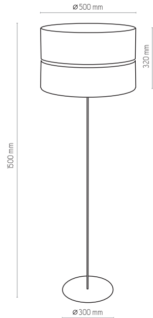
5465 | HILTON | 1x E27, 25W LED | AB 8998
