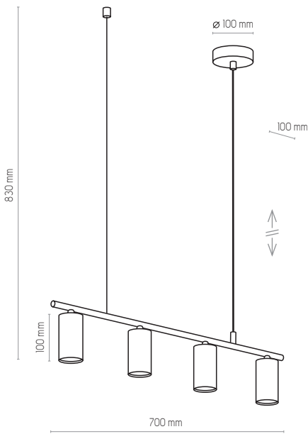
4427 | LOGAN BLACK | 4 x GU10, 10W LED
