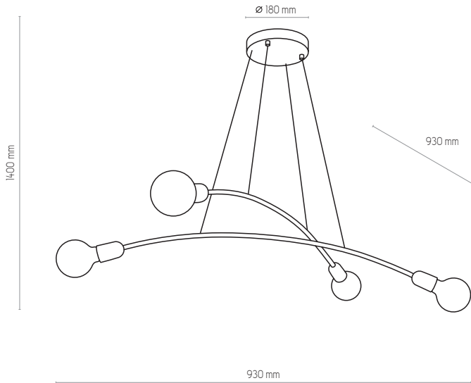
2727 | HELIX GOLD | 4 x E27, max 60W
