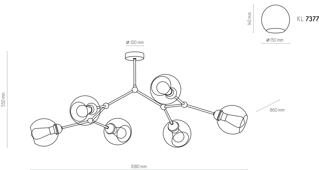
1979 | FAIRY GOLD | 6 x E27, max 60W
