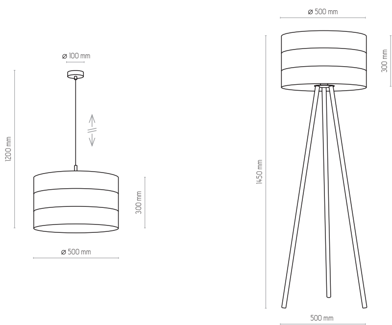
3211 | TAGO BLACK | 1x E27, 25W LED | AB 9036
