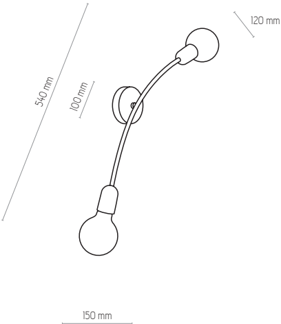
2719 | HELIX GOLD | 2 x E27, max 60W
