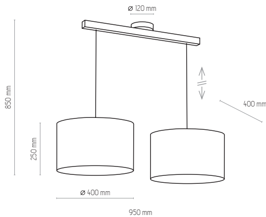
3373 | TROY WHITE | 2 x E27, 25W LED | AB 9168
