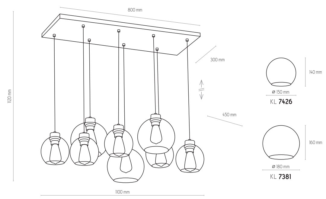
4113 | CUBUS GRAPHITE | 8 x E27, max 60W
