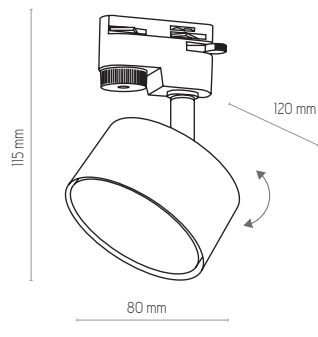
4397, 4398 | TRACER | 1 x GX53, 15W LED
