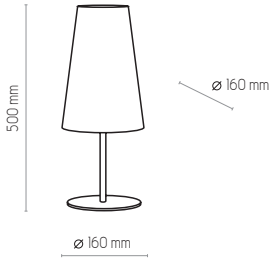
5169 | UMBRELLA | 1 x E27, 25W LED | AB 9088
