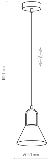
2320 | VICHY | 1 x GU10, 10W LED | KL 7808
