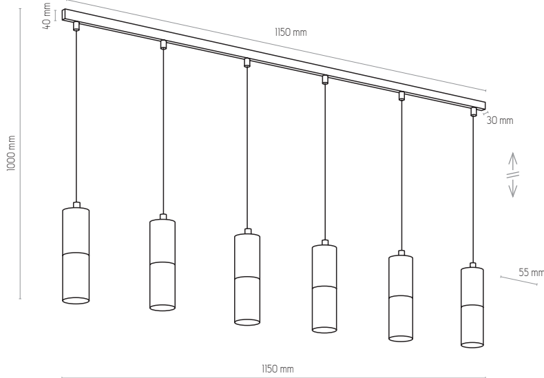
4368 | ELITE BLACK | 6 x GU10, 10W LED
