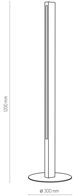
5043 | TEO | 1 x 230V, 30W, 3000K, 3270lm
