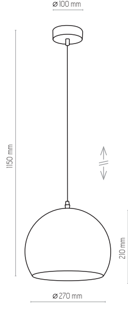
2085 | YODA BLACK ORBIT | 1 x E27, max 60W
