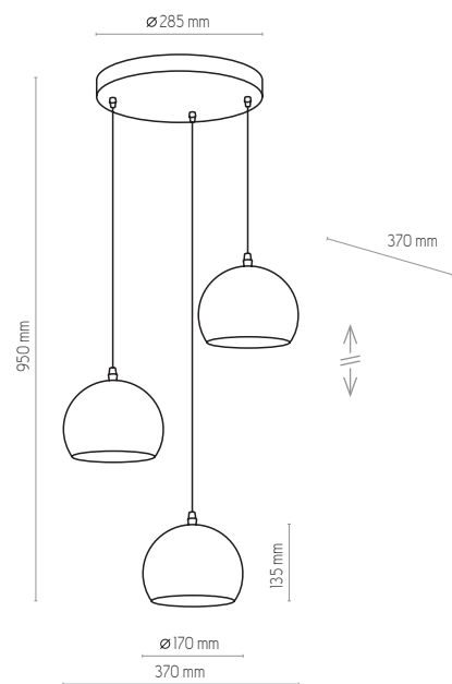
3448 | YODA GOLD ORBIT | 3 x E27, max 60W
