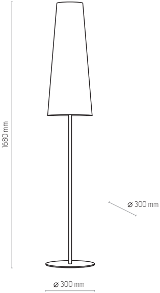
5176 | UMBRELLA | 1 x E27, 15W LED | AB 9095
