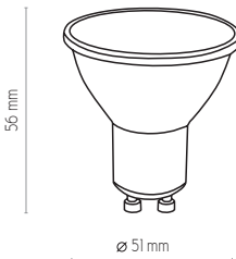
3577 | BULB LED | GU10. 4000K, 480lm, 220-240V, 50 HZ, 5W 3578 | BULB LED | GU10. 2700K, 350lm, 220-240V, 50 HZ, 5W
