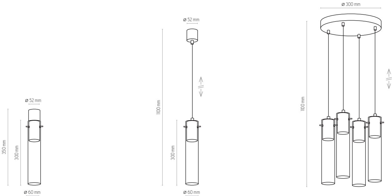
3147 | LOOK GRAPHITE | 1 x GU10, 10W LED | KL 4101
