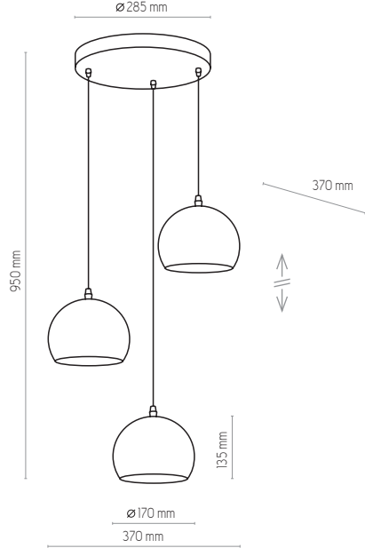
2082 | YODA BLACK ORBIT | 3 x E27, max 60W
