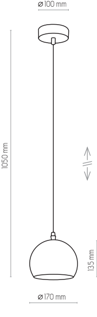
2080 | YODA BLACK ORBIT | 1 x E27, max 60W
