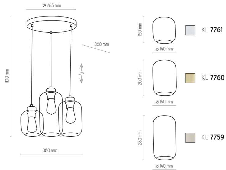
3175 | MARCO BROWN | 3 x E27, max 60W
