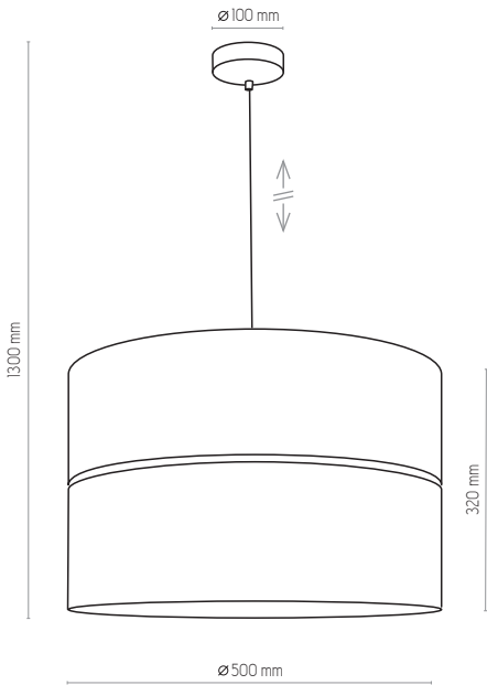
4346 | HILTON | 1 x E27, 25W LED | AB 8999
