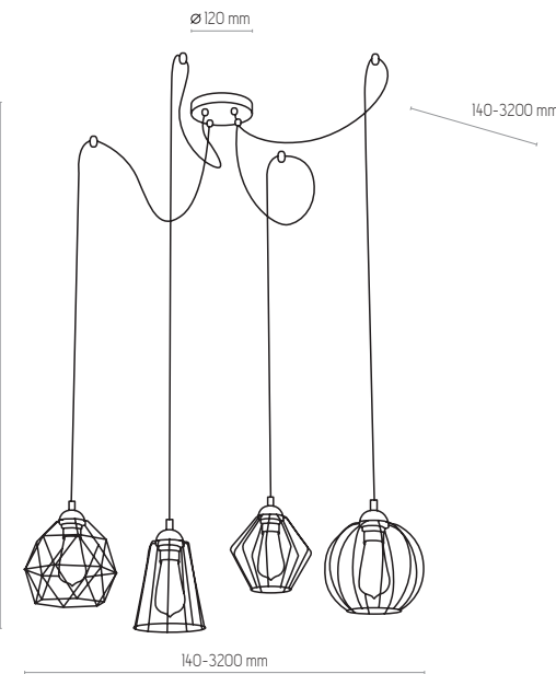
1646 | GALAXY | 1 x E27, max 60W | DM 4, DM 15, DM 16, DM 13
