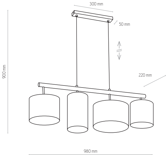
4106 | DEVA WHITE | 4 x E27, 15W LED | AB 8933
