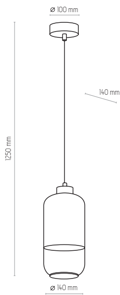
3356 | MARCO SILVER | 1 x E27, max 60W
