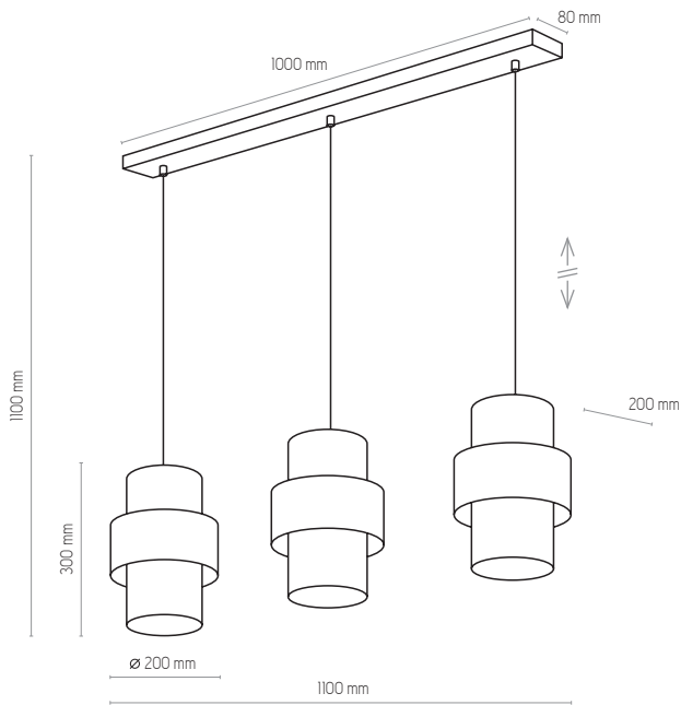
4378 | CALISTO | 3 x E27, 15W LED | AB 9083
