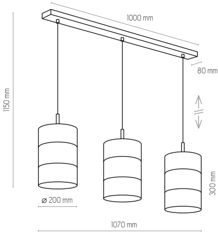
3215 | BOGART BLACK | 3 x E27, 15W LED | AB 9035
