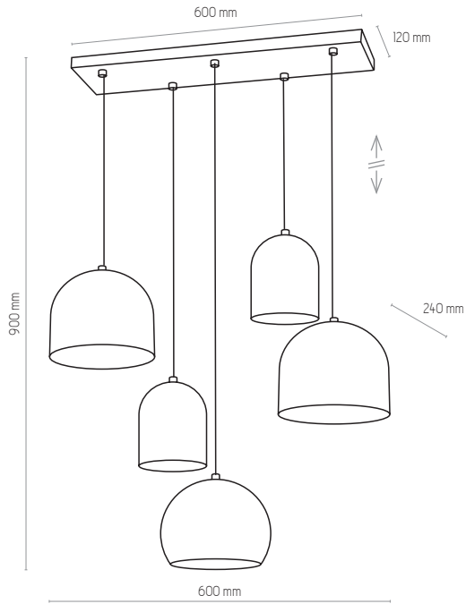
2829 | TEMPRE | 5 x E27, 15W LED
