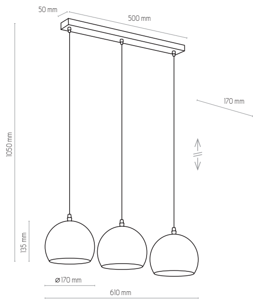
2081 | YODA BLACK ORBIT | 3 x E27, max 60W
