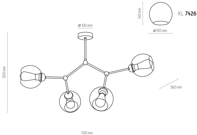
2730 | FAIRY | 4 x E27, max 60W
