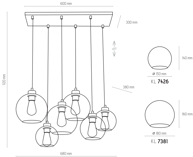
2833 | CUBUS GRAPHITE | 6 x E27, max 60W
