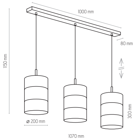
3209 | BOGART WHITE | 3 x E27, 15W LED | AB 9038
