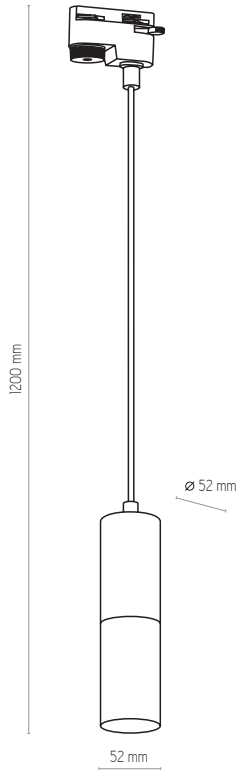
4402, 4403 | TRACER | 1 x GU10, 10W LED
