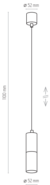
4366 | ELITE BLACK | 1 x GU10, 10W LED
