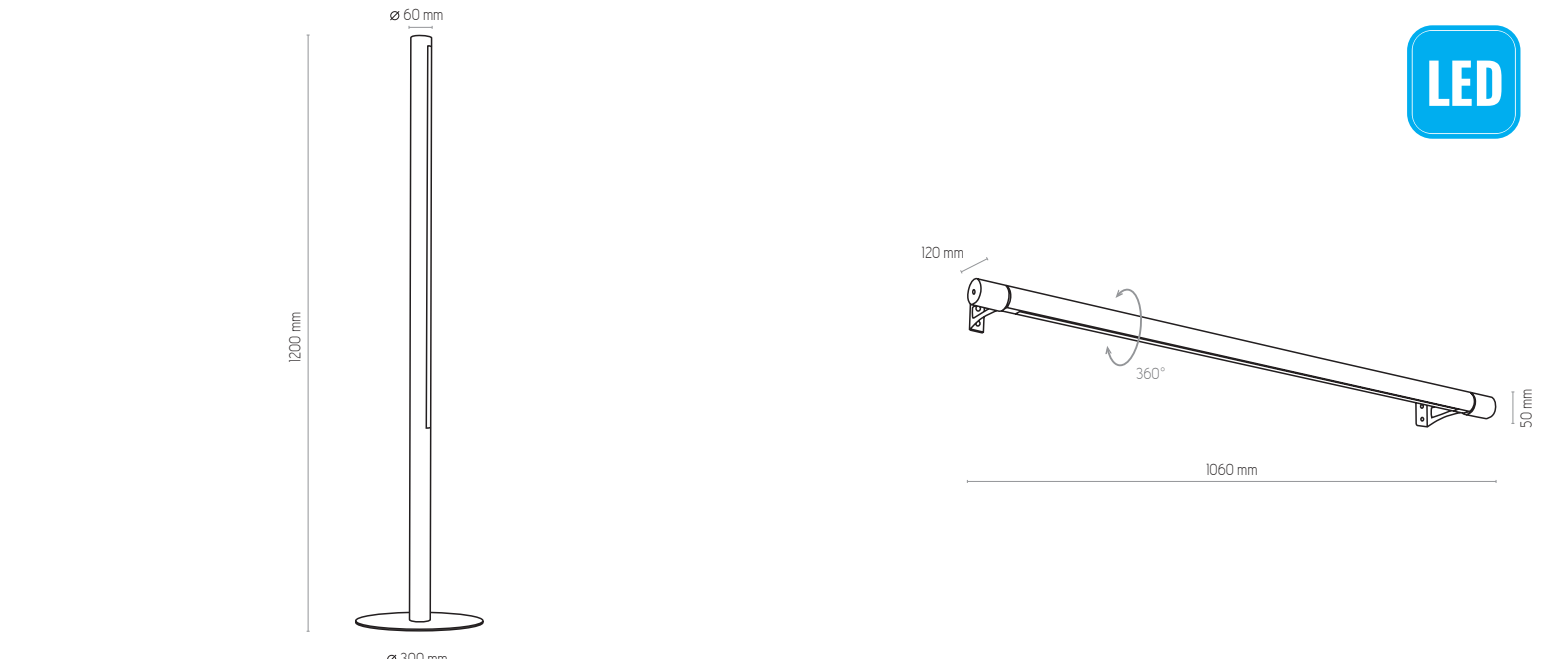
1409 | ROLLO | 1 x 230V, 30W, 3000K, 3250lm
