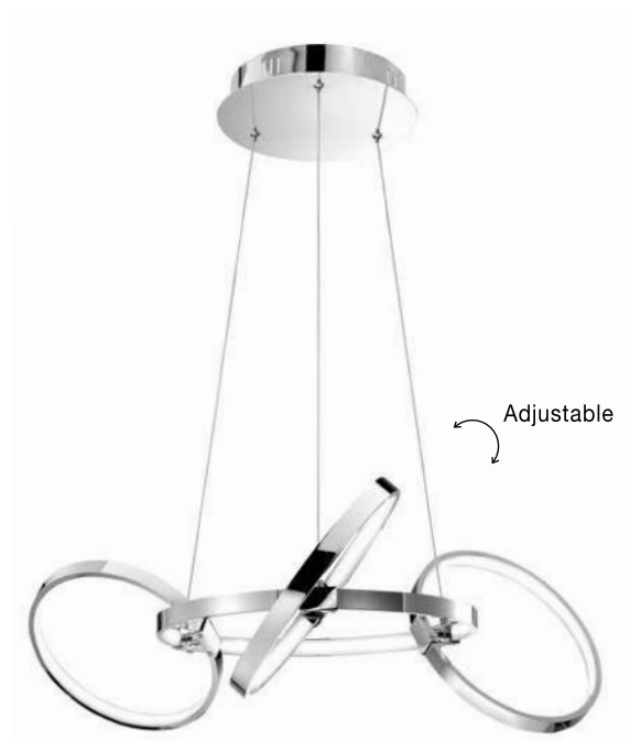
FOLIGNO - 7272801 Chrome Aluminium & Acrylic Adjustable LED 39 Watt 230 Volt 2340Lm 3000K IP20 Dimmable L: 74.5 H: 120 cm
