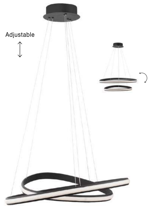
ARIES - 9357063 Dimmable Sandy Black Aluminium & Acrylic LED 48 Watt 230 Volt 2363Lm 3000K IP20 D: 59 H: 120 cm
