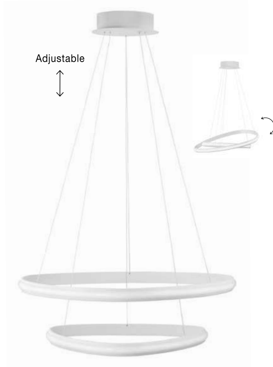
ARIES - 9357061 Dimmable Sandy White Aluminium & Acrylic LED 48 Watt 230 Volt 2363Lm 3000K IP20 D: 59 H: 120 cm
