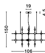
ATOMO - 9180630 Dimmable Gold Metal & Acrylic LED 30 x 2.4 Watt 230 Volt 5040Lm 3000K IP20 L: 106 W: 58.5 H: 150 cm Included Remote Control
