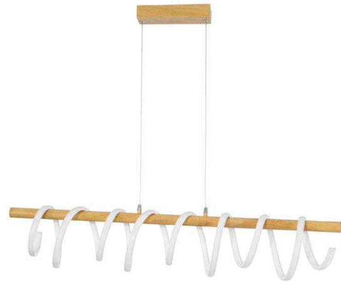
MIRCO - 9071010 Dimmable Wood Colour White Aluminium & Acrylic LED 38 Watt 3 Volt 2650Lm 3000K IP20 L: 100 W: 23 H: 150 cm LED WARM WHITE A++ A DRIVER INCL.
