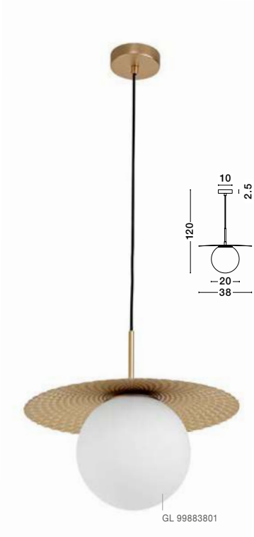
OBBIT - 9988381 Opal Glass Gold Metal LED E27 1x12 Watt 230 Volt IP20 Bulb Excluded D: 20 H: 32 H 2 : 120 cm
