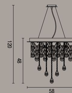
sospensione Hemidark Hemidark pendant lamp
