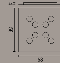
plafoniera Flet 8 luci Flet ceiling lamp with 8 lights
