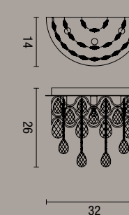
applique Hemidark Hemidark wall lamp
