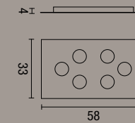
plafoniera Flet rettangolare 6 luci Flet rectangular ceiling lamp with 6 lights
