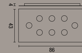
plafoniera Flet rettangolare 8 luci Flet rectangular ceiling lamp with 8 lights
