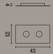
plafoniera Flet rettangolare 2 luci Flet rectangular ceiling lamp with 2 lights
